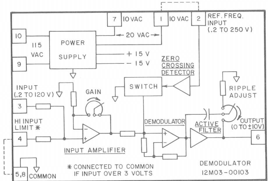
FIGURE 1 SIMPLIFIED SCHEMATIC
